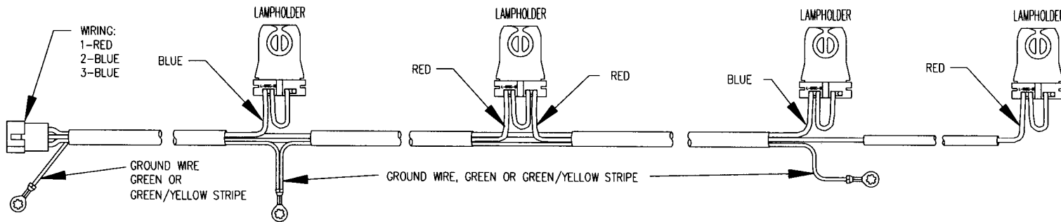
20718, HARNESS, DUAL LAMP 110V
